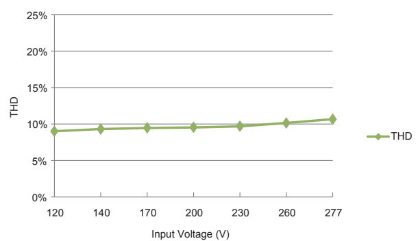
THD vs Input Voltage
