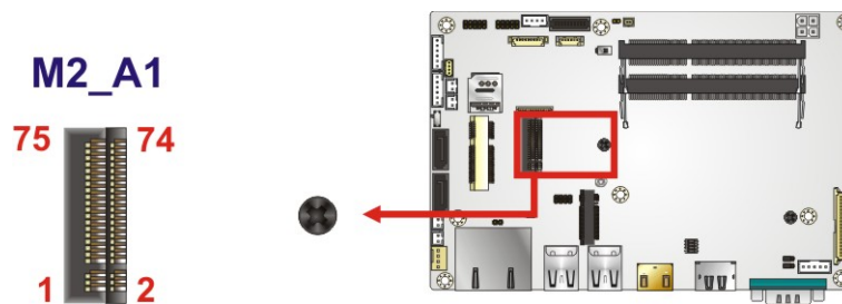
Figure 3-11: M.2 A-key Slot Location
