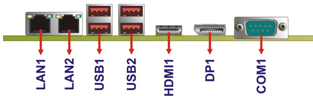
Figure 3-27: External Peripheral Interface Connector
